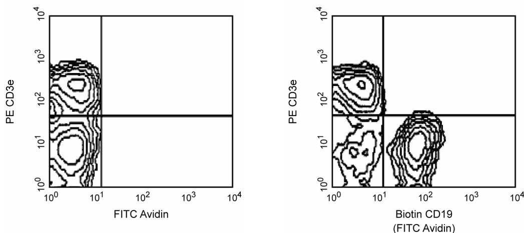
Two-color analysis of the expression of CD19 on mouse spleen B cells. BALB/c splenocytes were stained with PE-conjugated anti-mouse CD3e mAb 145-2C11 (Cat. No. 553063) in the absence (left panel) or presence (right panel) of biotin-conjugated 1D3 mAb followed by Avidin-FITC (Cat. No. 554057). Flow cytometry was performed on a BD FACScan™ flow cytometry system.
